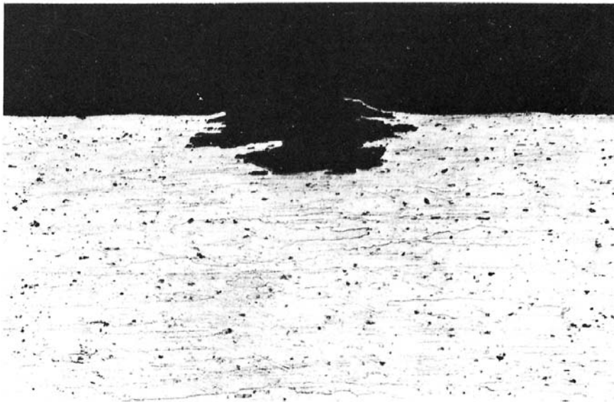
Undermining pitting that may form the surface give the appearance of incipient exfoliation (Keller's Etch; 100x).
